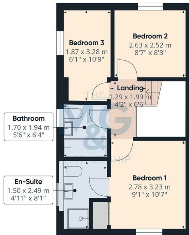
Floor 1 Building 1
